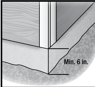
Figure 13 Block Penetration
