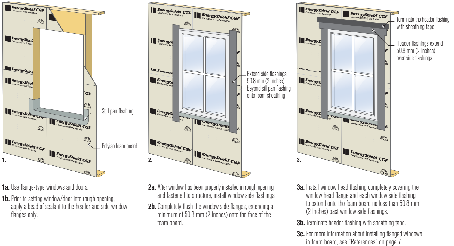
FIGURE A: FLANGED WINDOW INSTALLATION
